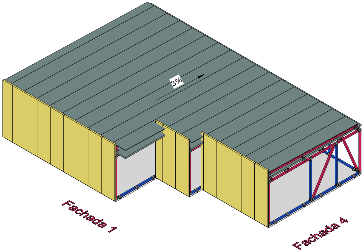
2 3D Fachada 1 P-03
