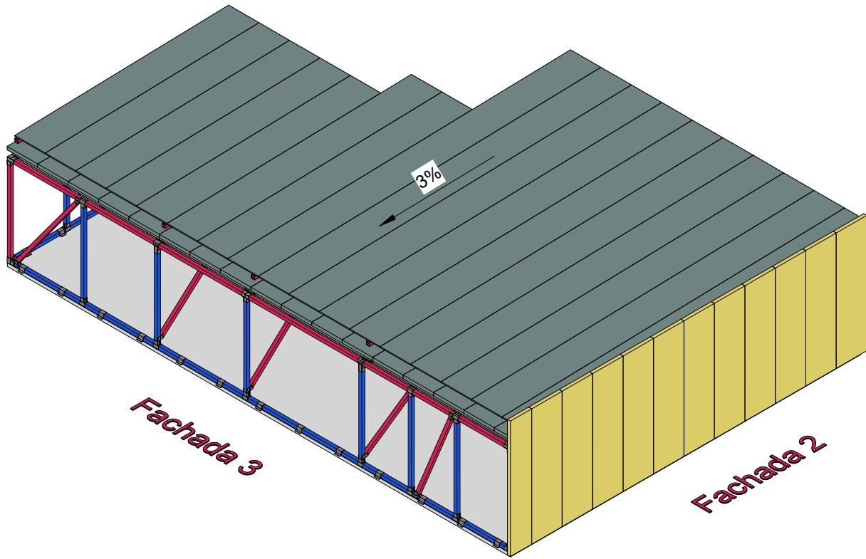
2 3D Fachada 2 P-04
