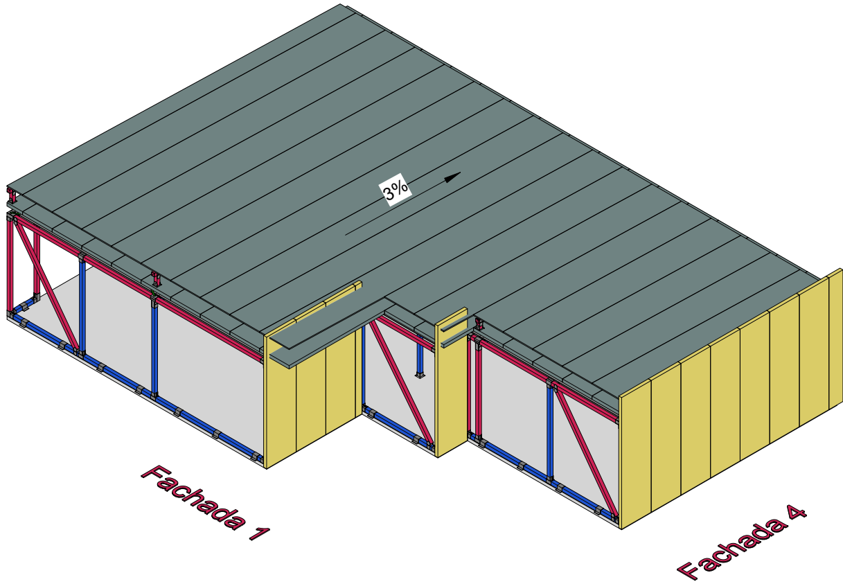
2 3D Fachada 4 P-06
