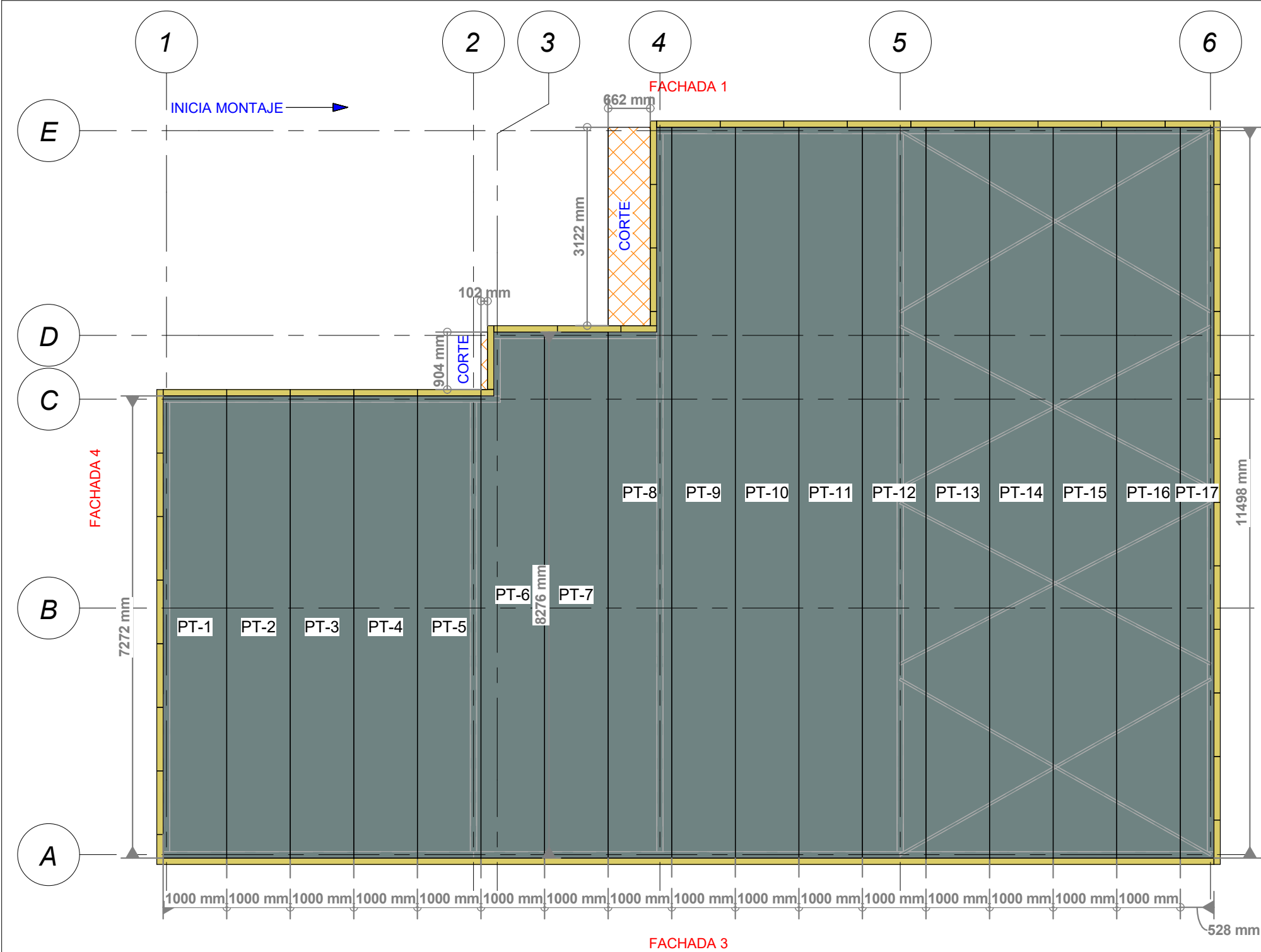
1 Paneles Tapa P-01 1 : 75
