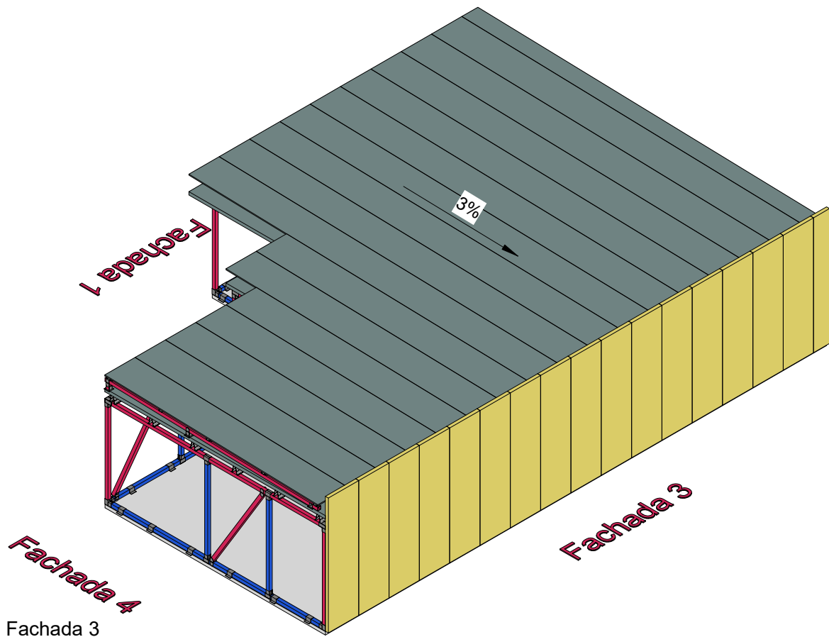
2 3D Fachada 3 P-05
