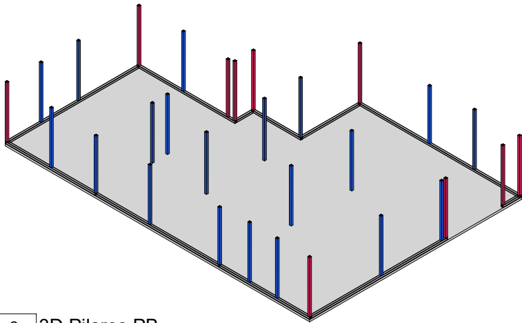
2 3D Pilares PB T-02
